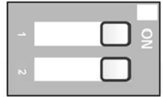
Original Software Switch Position for Non-W204 Vehicles
